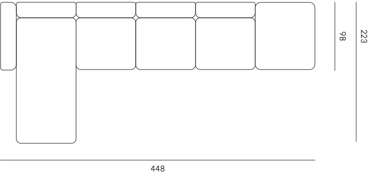
Divano 3 posti con chaise longue e allunga 3 seats sofa with chaise longue and extension
