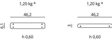
Piastre / Plates
